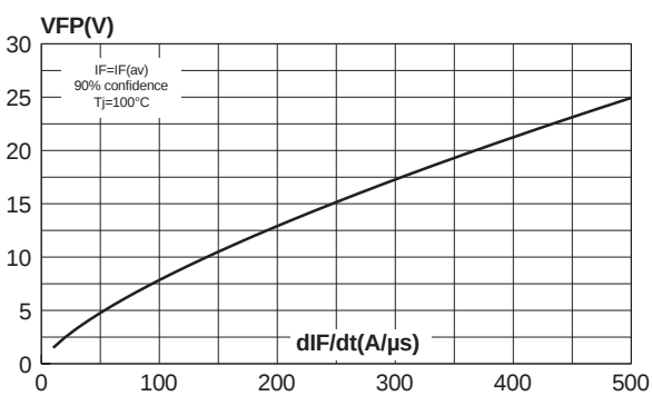
Fig. 10: Transient peak forward versus dI_F/dt (per diode).
